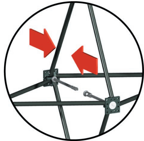
4. Locking detail
